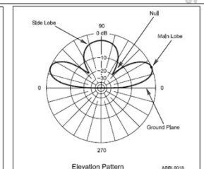
Figure 4.6 — The elevation pattern looks at the antenna from the side to see how well it receives and transmits at different angles above a horizontal plane.
