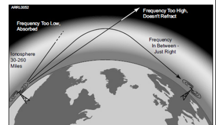
Fig 4.2: Signals in the right range of frequencies are refracted back toward the Earth and are received hundreds or thousands of miles away.
