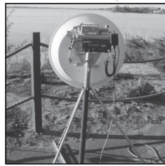
Figure 4.14 — N7CFO's dish antenna operates on 10 GHz and is portable enough to be taken on contest outings.
