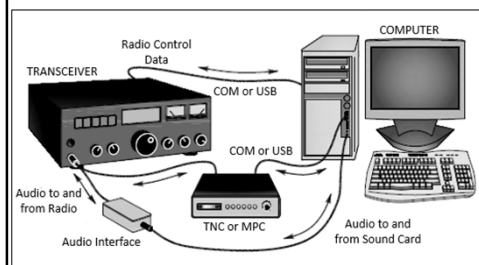
Figure 5.10 ... Typical Digital Mode Set Up
