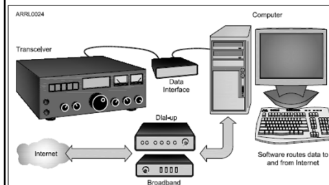
Figure 5.11 ... Typical Gateway Set Up
